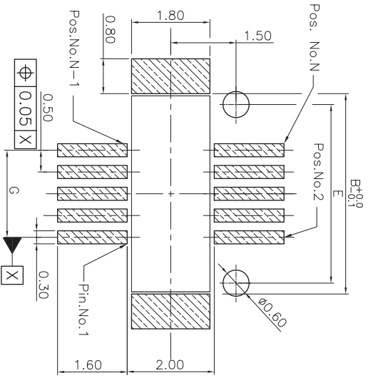
RECOMMENDED PCB LAYOUT TOLERANCE: + / - 0.03
